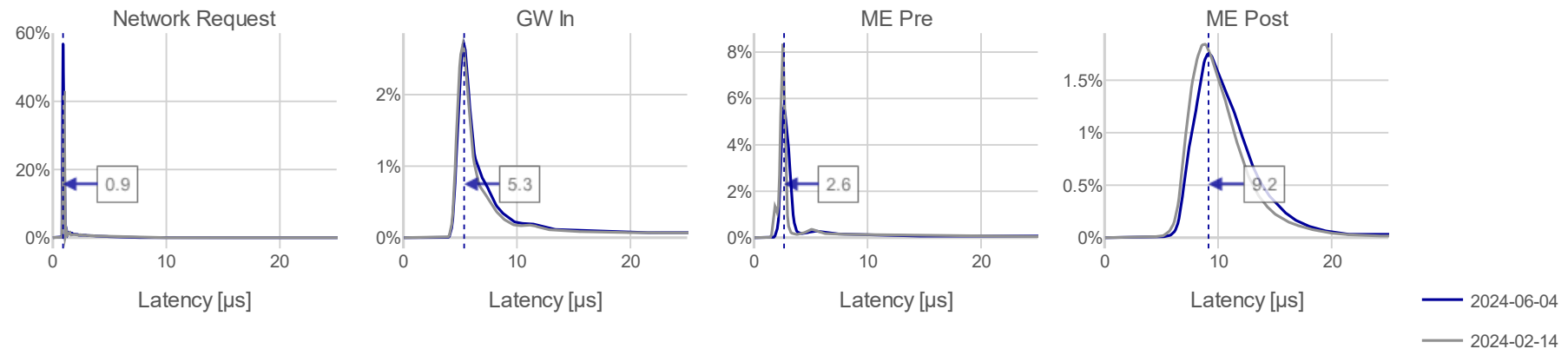
Futures latency compared with 2024-02-14
